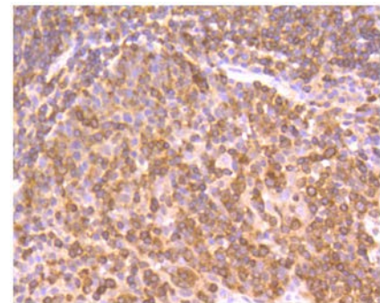
Fig. 2. Immunohistochemical analysis of paraffin-embedded human tonsil tissue using anti-NFkB p105/p50 antibody. Counter stained with hematoxylin.
